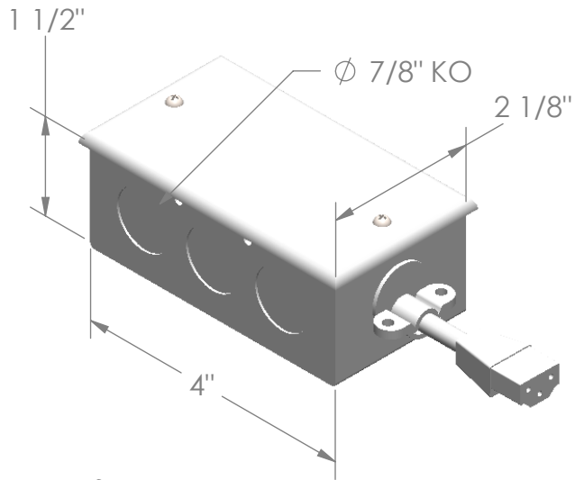
DLN31FA1 WHITE HARDWIRE BOX DIMENSIONS: 4"L x 2 1/8"W x 1 1/2"H 11 X Ø 7/8" KOs
